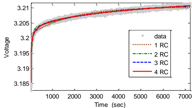
Figure 5: Curve fit to determine number of R-C branches.
