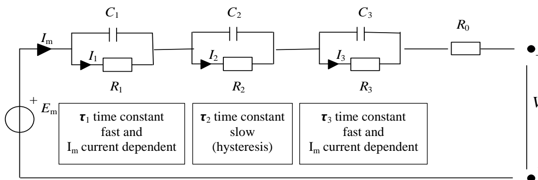
Figure 7: Equivalent circuit model with 3 R-C branches.
